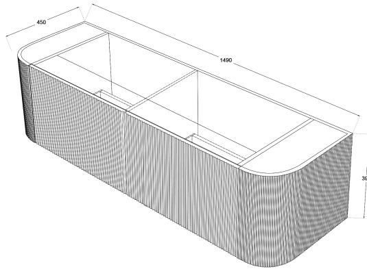
TOP VIEW: DRAWERS
