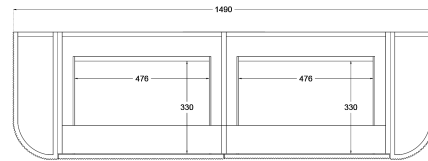
SIDE VIEW: DRAWER STORAGE
