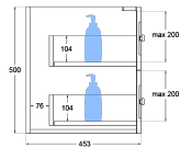
SIDE VIEW: DRAWER STORAGE
