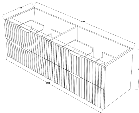
TOP VIEW: DRAWERS
